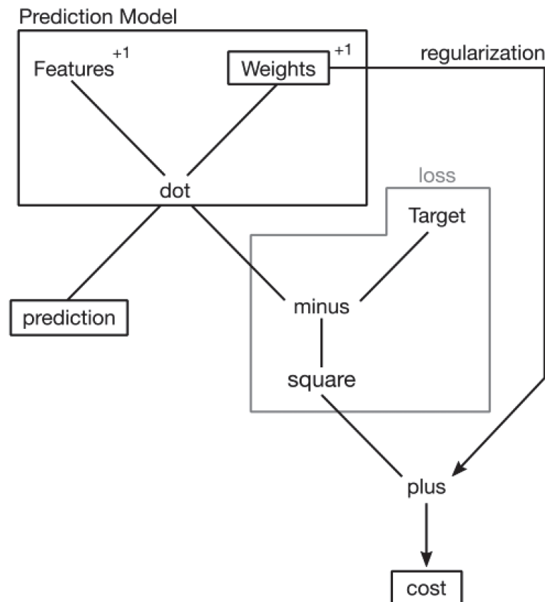
Figure 15.1 A graphical view of linear regression.
