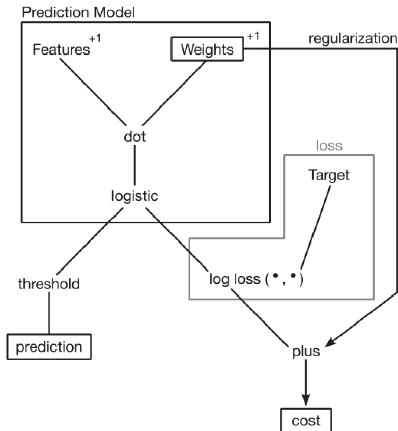
Figure 15.2 A graphical view of logistic regression.
