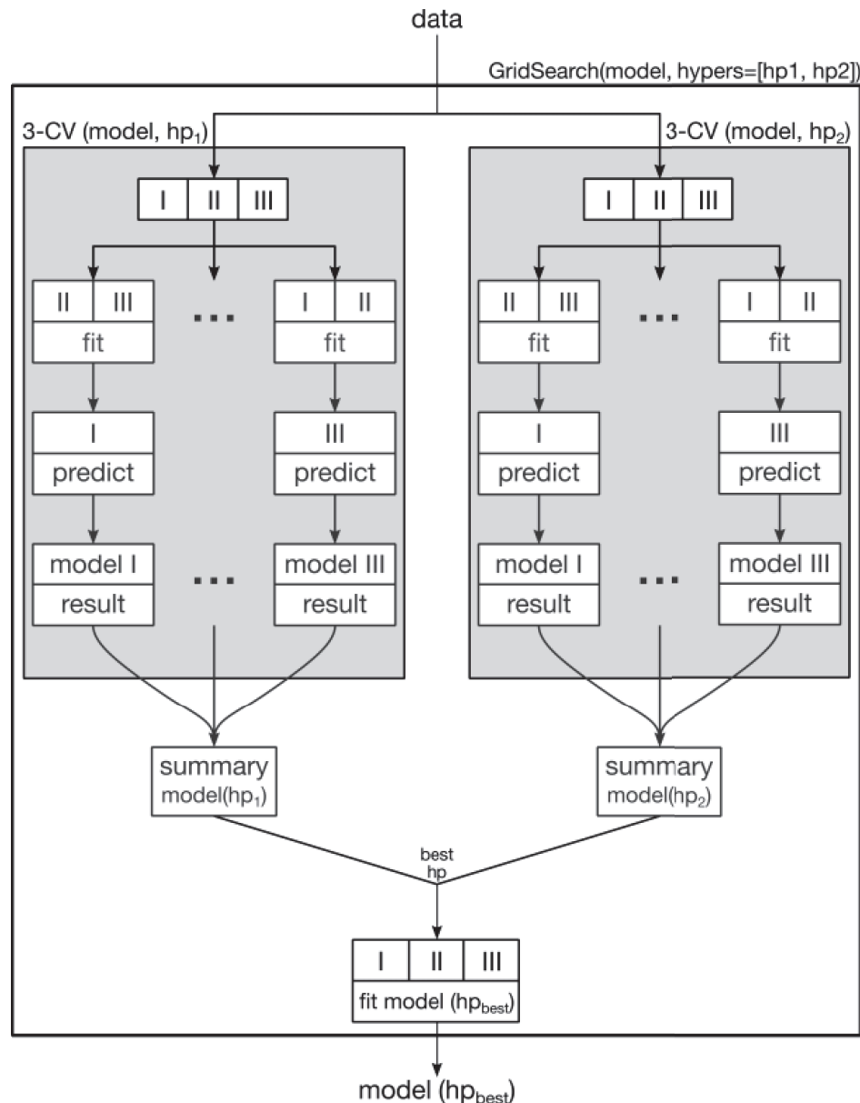
Figure 11.3 GridSearch.
