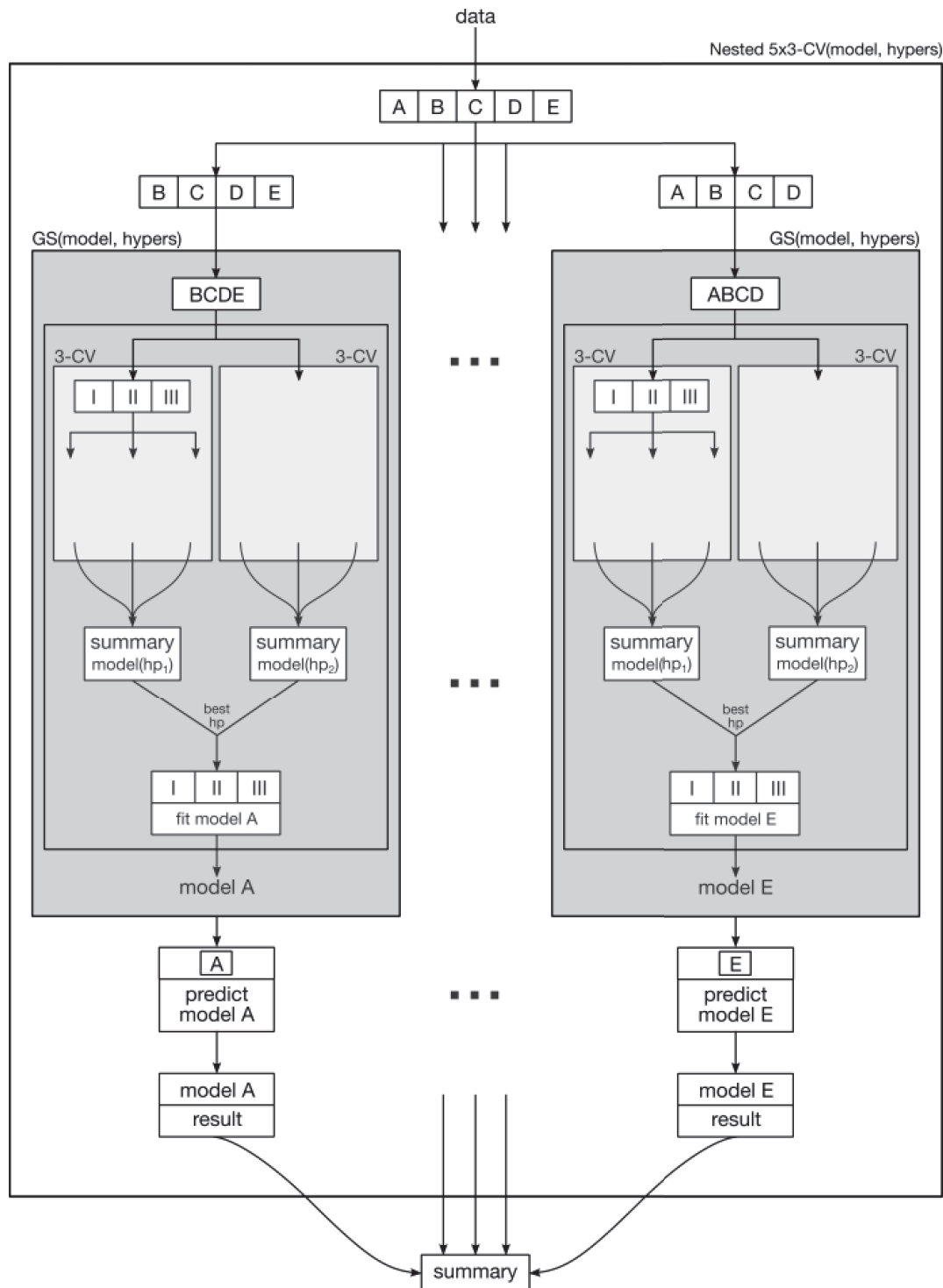
Figure 11.4 Nested cross-validation for GridSearch.
