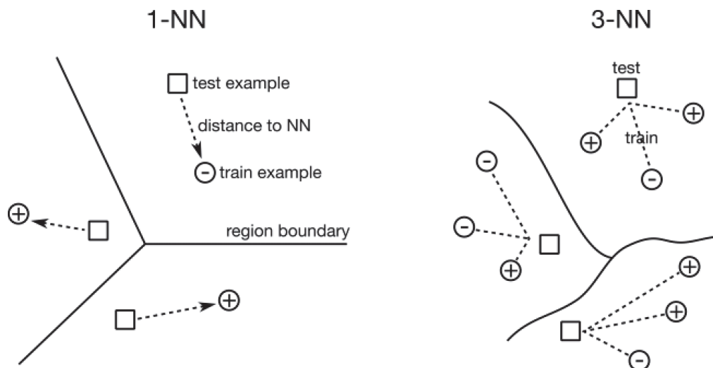
Figure 5.9 Bias in k -NN.
