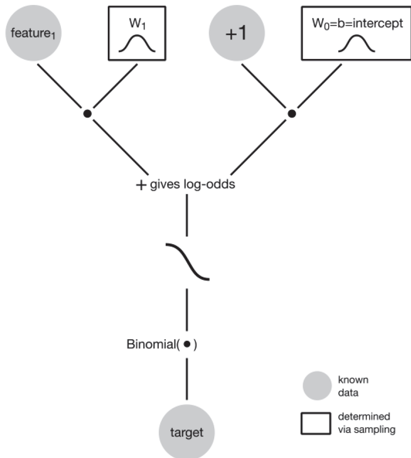
Figure 15.7 A probabilistic graphical model for logistic regression.
