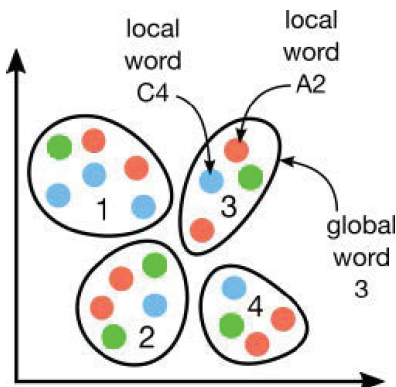
Figure 14.4 Creating the global vocabulary.
