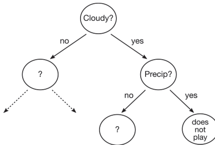
Figure 8.2 A simple decision tree.
