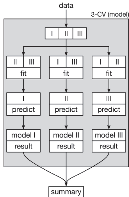
Figure 11.1 Flat cross-validation on a generic model.
