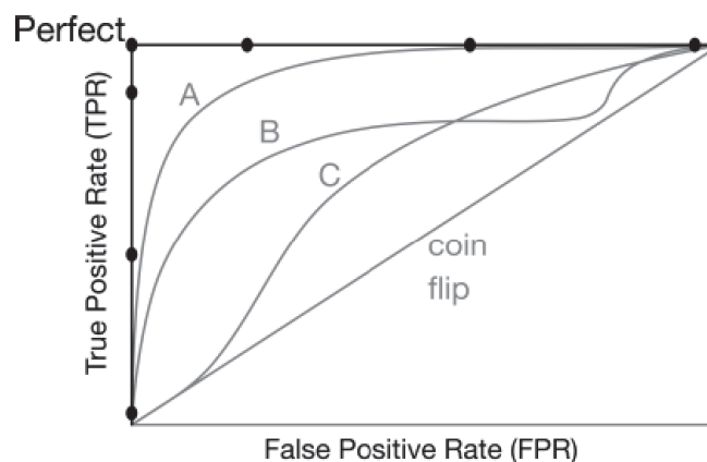
Figure 6.4 An abstract look at an ROC curve.
