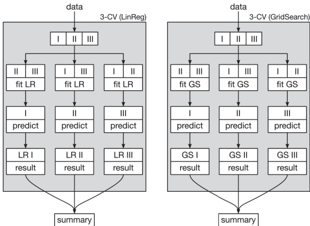
Figure 11.2 Wrapping models in cross-validation.
