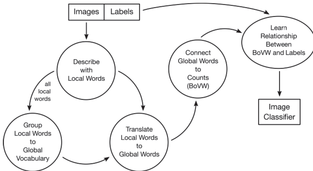
Figure 14.1 Outline of our image labeling system.
