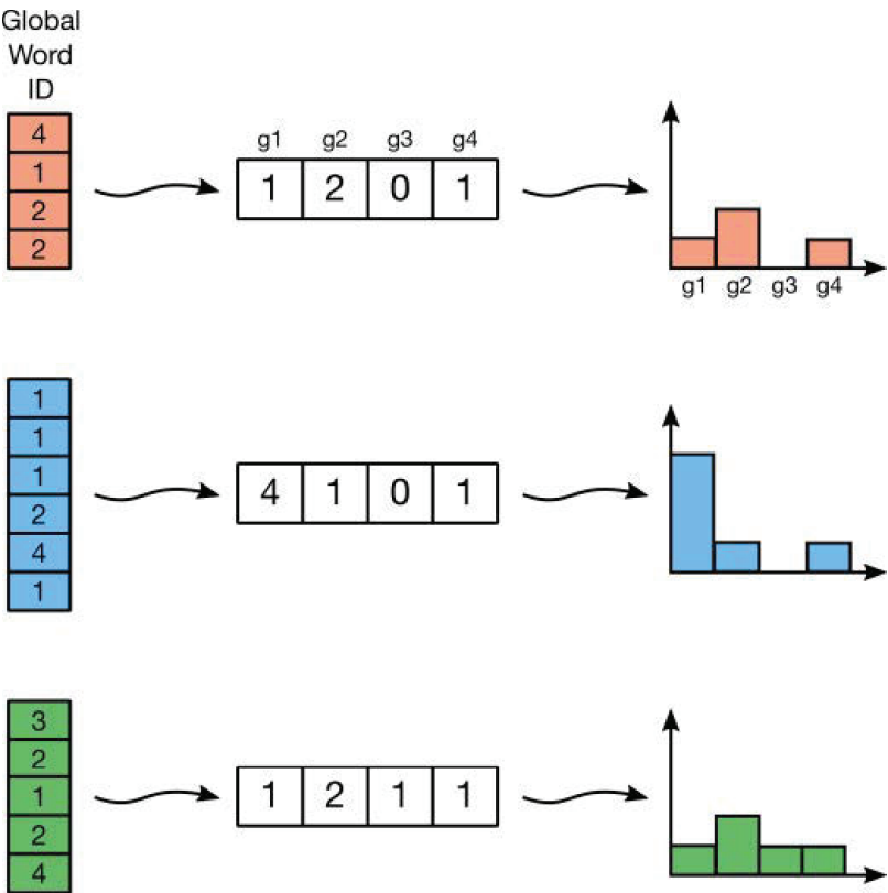
Figure 14.6 Collecting global vocabulary counts as histograms.
