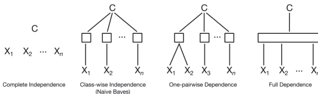
Figure 5.12 Naive Bayes is one bias-variance point on a spectrum of possibilities.
