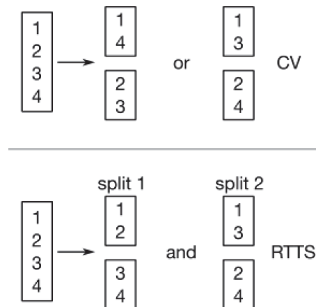
Figure 5.8 RTTS may have duplication between repeats.
