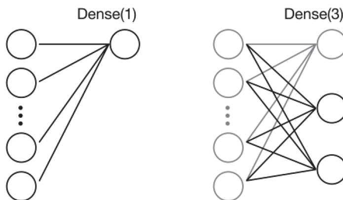
Figure 15.5 Dense layers.
