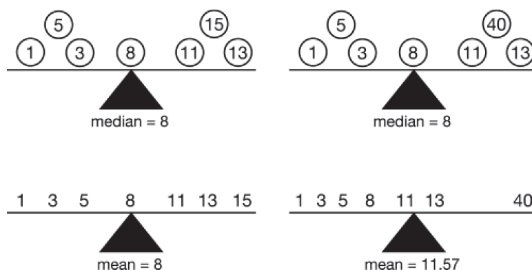
Figure 4.1 Comparing mean and median with balances.
