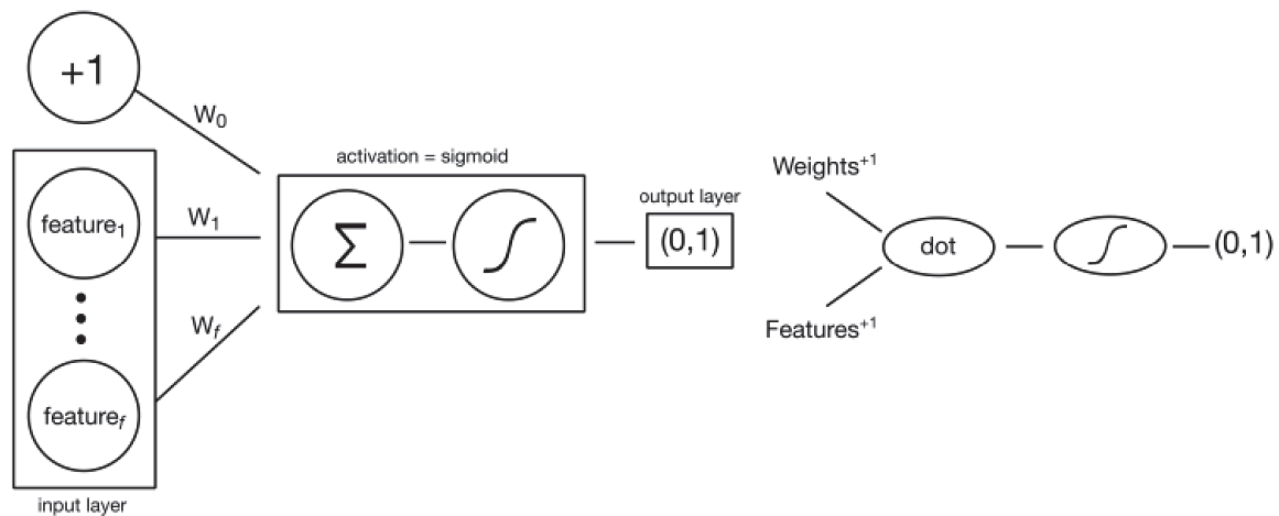
Figure 15.4 A neural network view of logistic regression.
