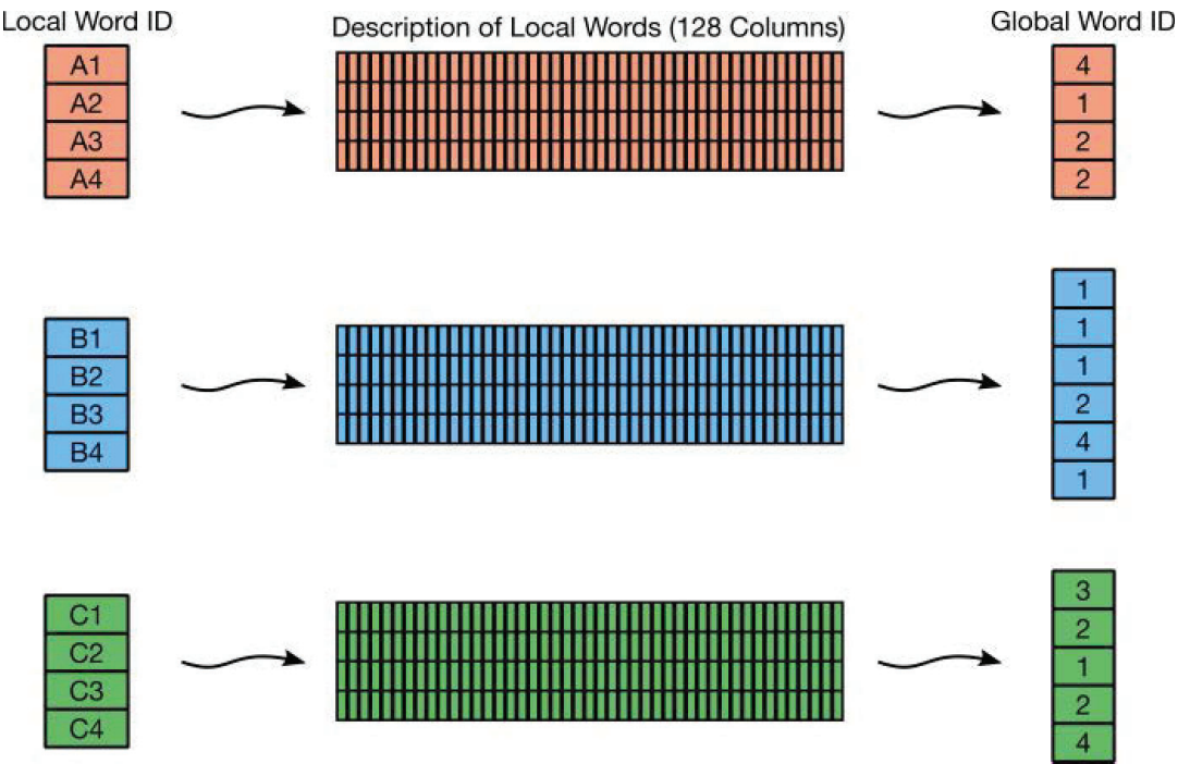
Figure 14.5 Translating local words to the global vocabulary.
