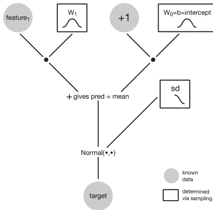
Figure 15.6 A probabilistic graphical model for linear regression.
