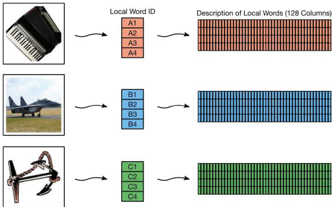
Figure 14.3 Extracting local visual words from the images.
