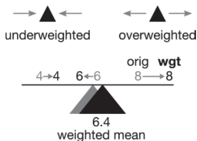
Figure 4.2 The effects of weighting on a mean.
