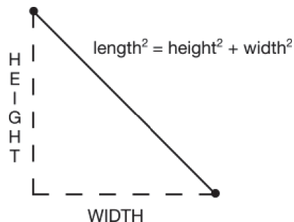
Figure 3.4 Distances from components.
