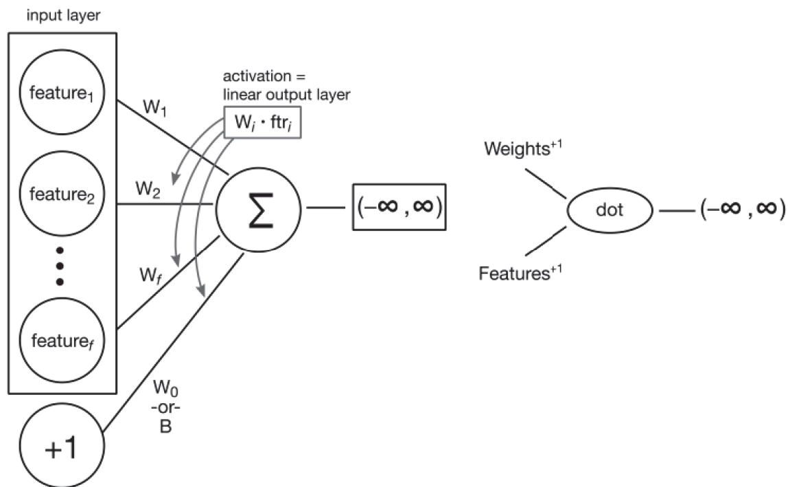
Figure 15.3 A neural network view of linear regression.
